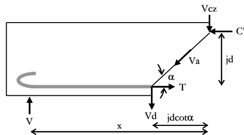
Figure 7: Forces within the shear span of an RC beam element without stirrups
