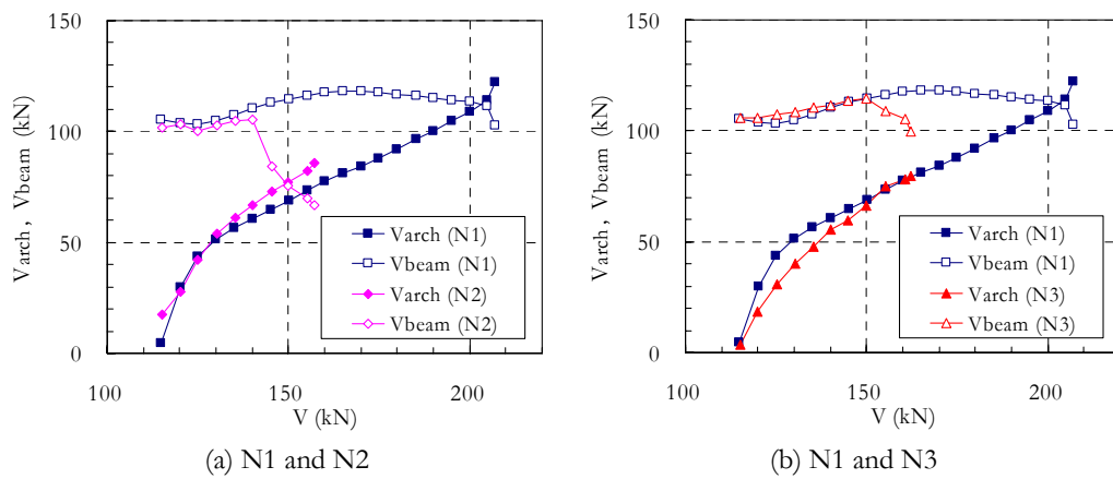
Figure 8: Comparison of the shear resisting forces by the arch and beam actions
