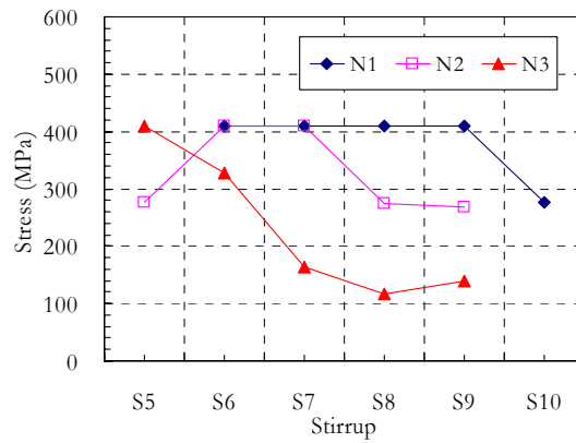
Figure 6: Stresses in stirrups employed for calculating their strength contribution
