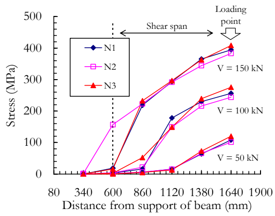
Figure 9: Stresses in main bars
