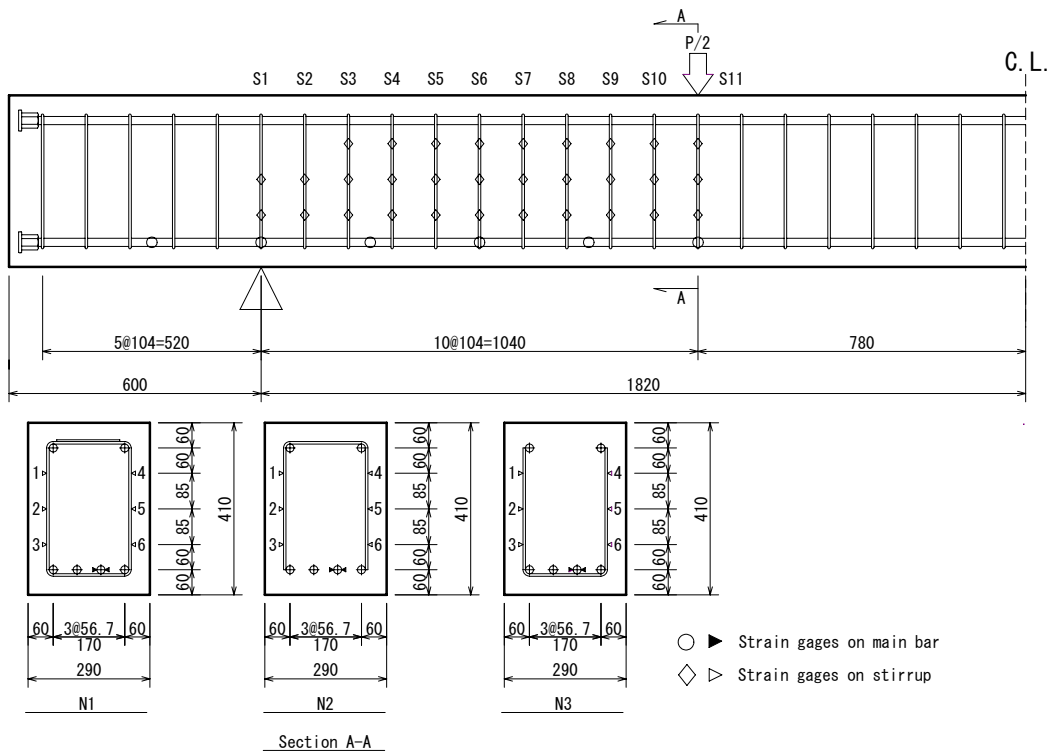
Figure 2: Specimen details (unit: mm)
