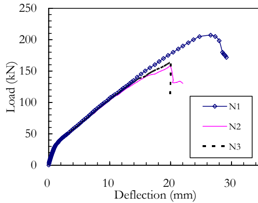
Figure 3: Load-deflection curve
