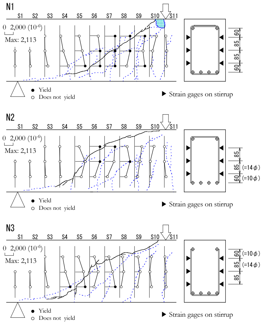
Figure 4: Strains in stirrups with crack patterns at the shear failure
