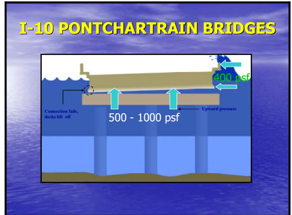
Figure 18 – Wave forces
