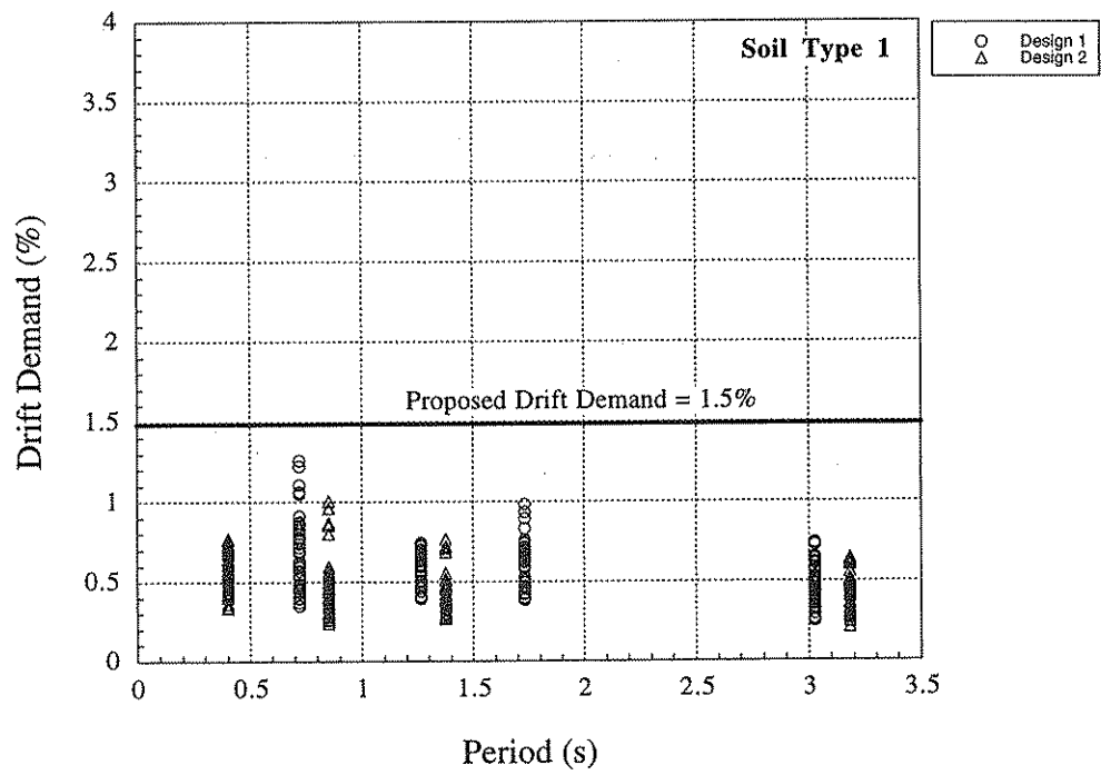
Figure 2. Drift Demand for UBC Soil Type 1.
