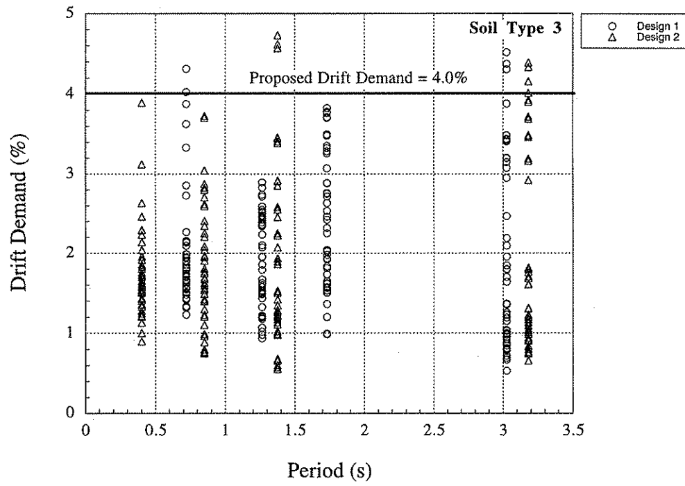
Figure 4. Drift Demand for UBC Soil Type 3.
