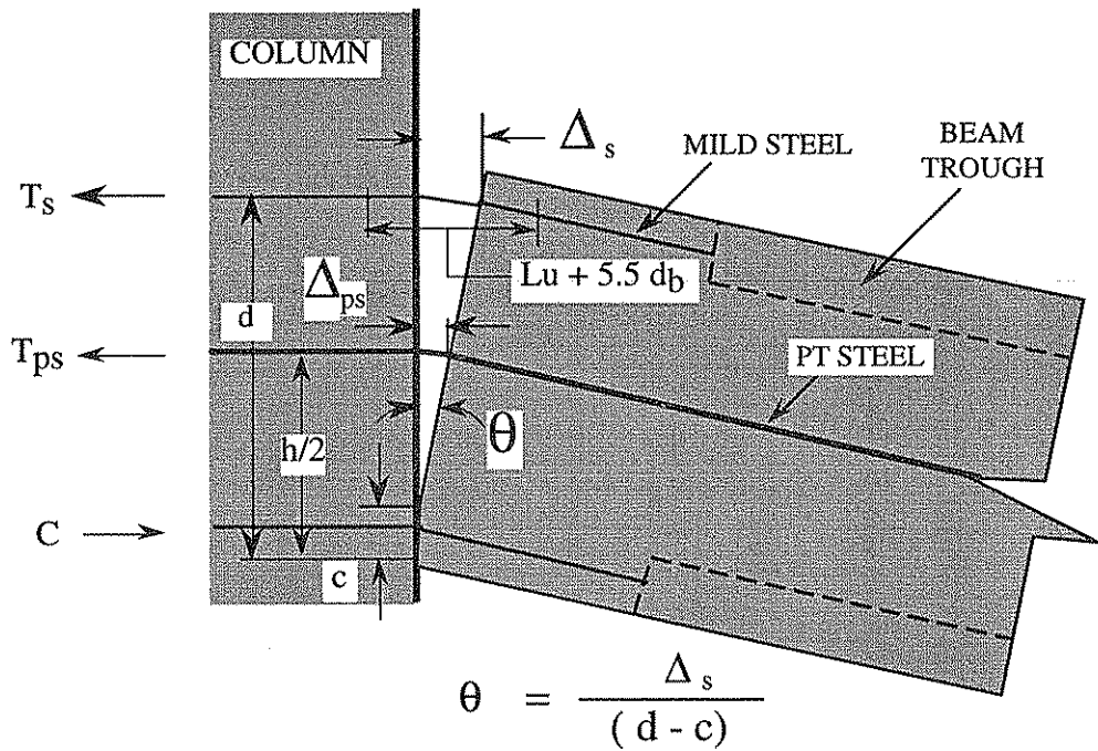
Figure 5. Rotation at the Beam-Column Joint.
