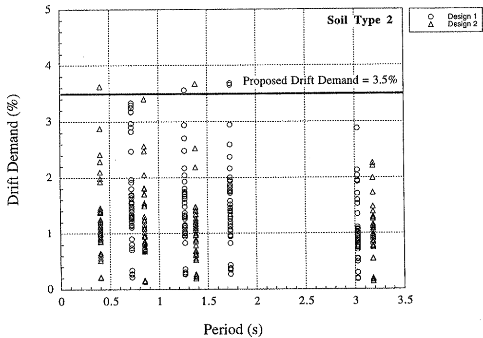
Figure 3. Drift Demand for UBC Soil Type 2.
