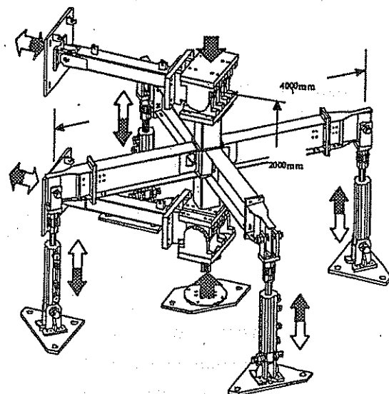
Fig.4 Diagonal Loading Test
