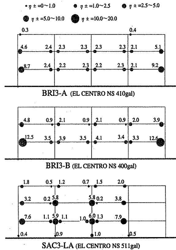
Fig.7 Damage Distribution ( V_t=150\text{kine} )
