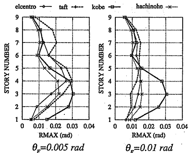
Fig.3 Maximum Interstory Drift Angles
