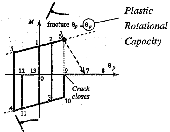
Fig.2 Hysteresis Model of Plastic Hinges at Beam-ends
