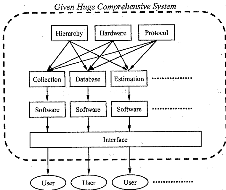
Figure 2.1 Top-down Approach
