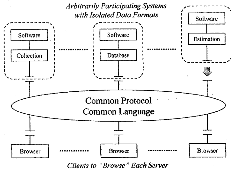
Figure 2.3 Bottom-up Approach
