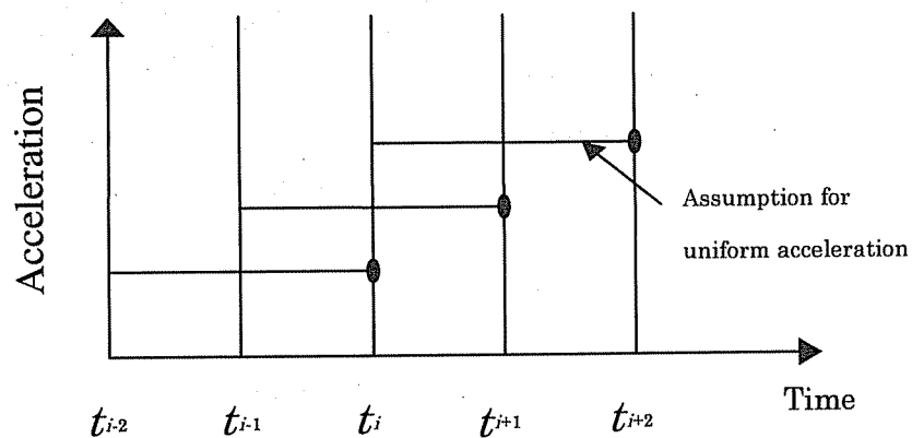
Figure-2 Assumption of acceleration in the central difference method
