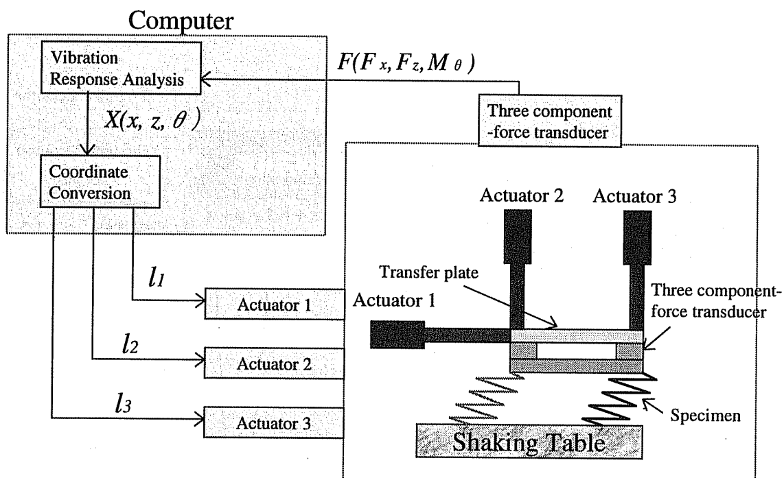
Figure-3 Concept of multi-axial hybrid vibration experiment system
