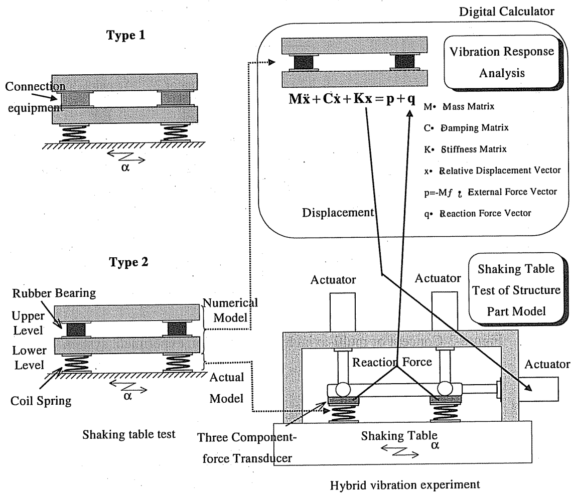
Figure-1 Conceptual view of hybrid vibration experiment
