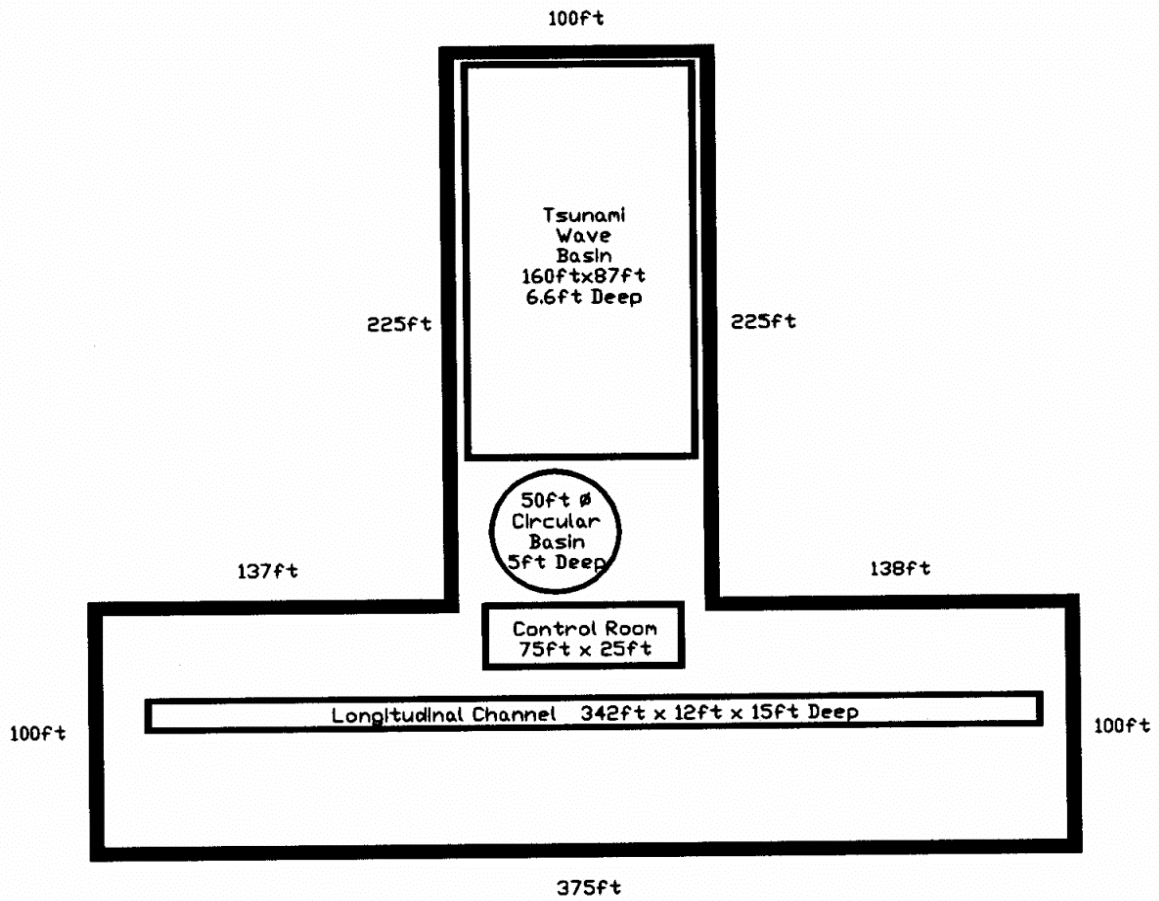
Figure 1. Plan view of the Oregon State Wave Research Laboratory.
