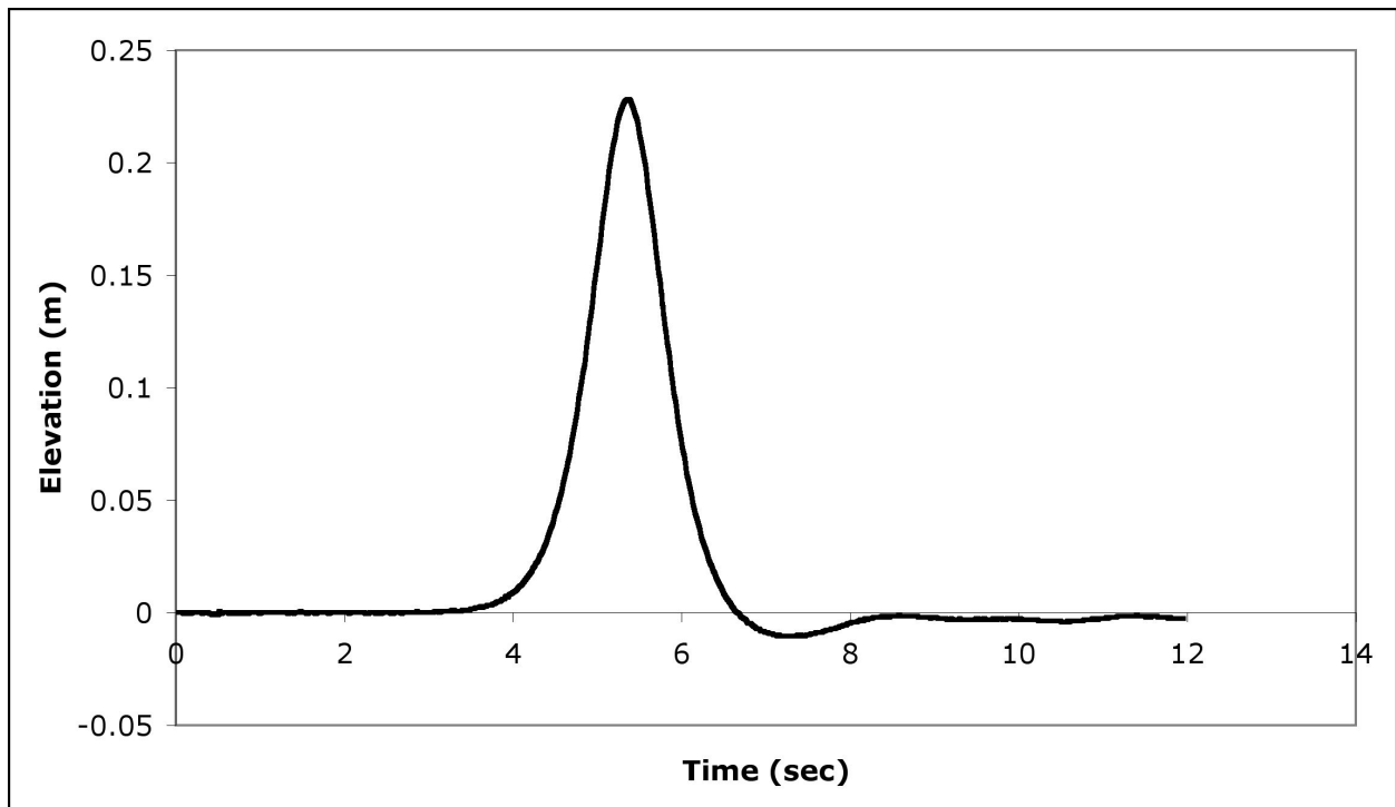
Figure 3. Generated solitary wave at 15.7 m from the waveboards. The targeted wave height is 0.24 m in 0.8m water depth.
