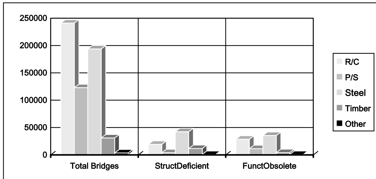
Figure 1: U.S. Bridge Distribution by Material and Deficiency
