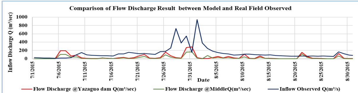
Figure 4. Comparison of flow discharge results between model and real field observed
