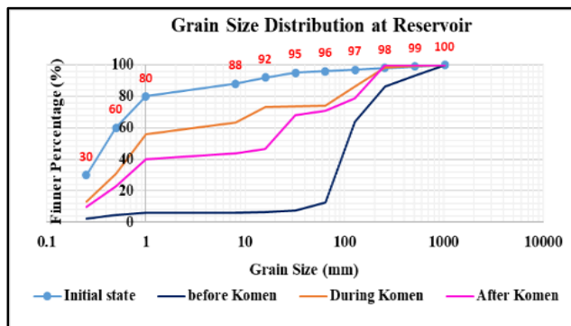
Figure 5. Sediment grain size distribution result
