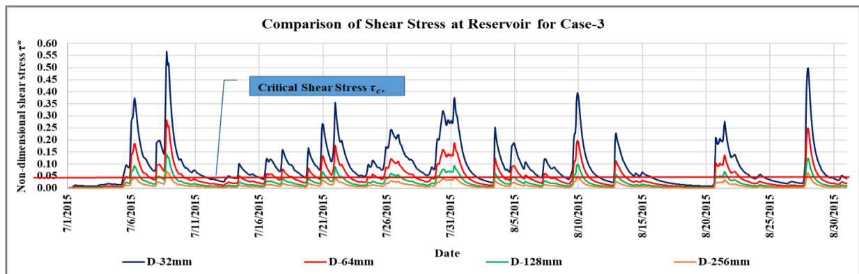
Figure 4. Comparison of shear stress at the reservoir
