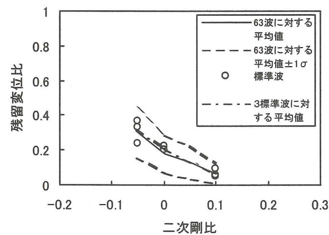
(c) \mu=6
