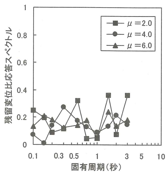
(b) r = 0
