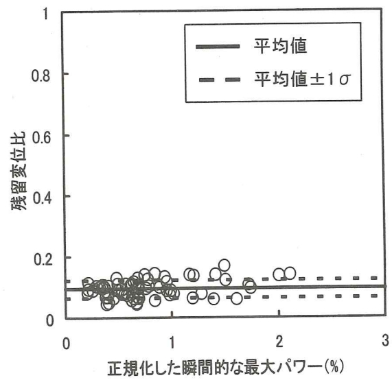
(b) \mu = 4
