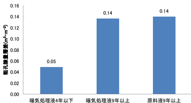
図40 施用年数別の粗孔隙量層差
